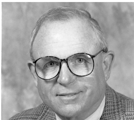
JIM BREAUT Founder of Television Production at Ferris State
